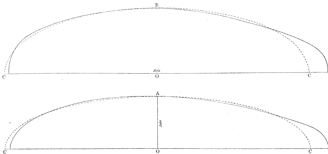
Second approximation to Pear-shaped Figure. Upper section "equatorial," lower "meridional."
